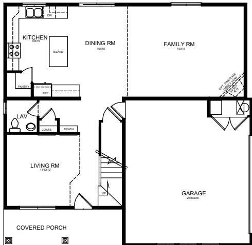
MAIN FLOOR PLAN 1000 S.F.
