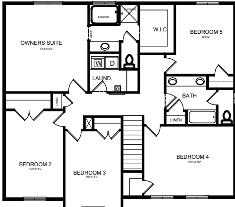
SECOND FLOOR PLAN 1140 S.F.
