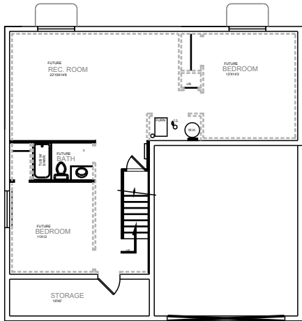
MAIN FLOOR PLAN 1000 S.F.
