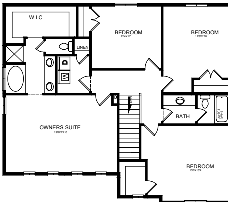
SECOND FLOOR PLAN 1290 S.F.
