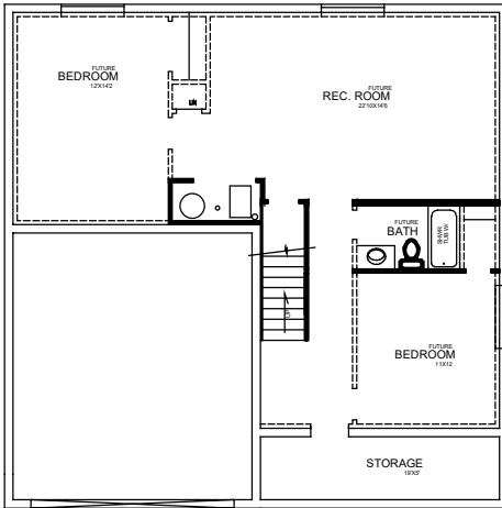
BASEMENT FLOOR PLAN 958 S.F.
