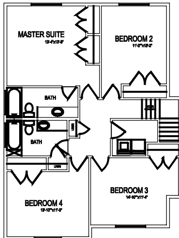
SECOND FLOOR PLAN 1128 S.F.
