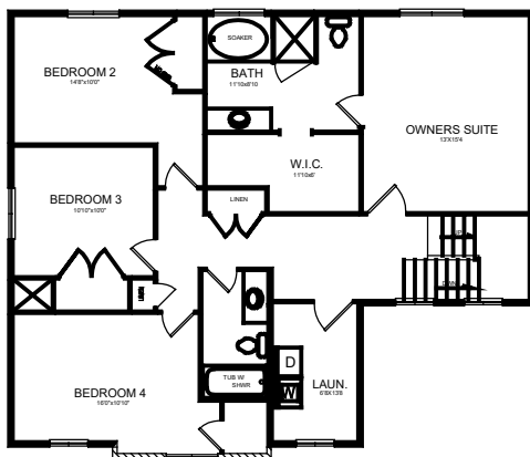
SECOND FLOOR PLAN 1260 S.F.
