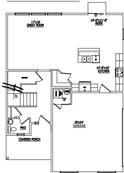
MAIN FLOOR PLAN 889 S.F.
