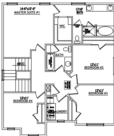
SECOND FLOOR PLAN 1,204 S.F.
