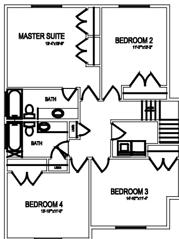
SECOND FLOOR PLAN 1128 S.F.
