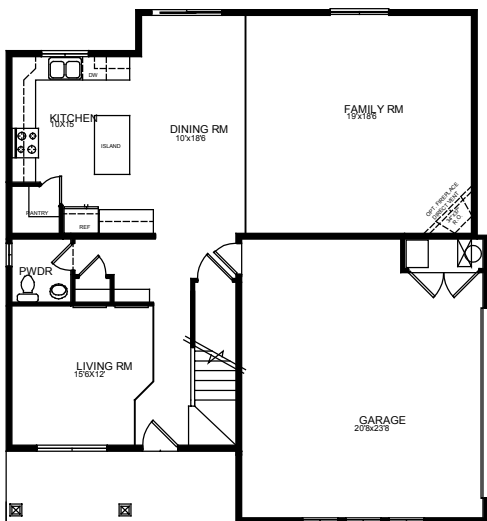
MAIN FLOOR PLAN 1102 S.F.
