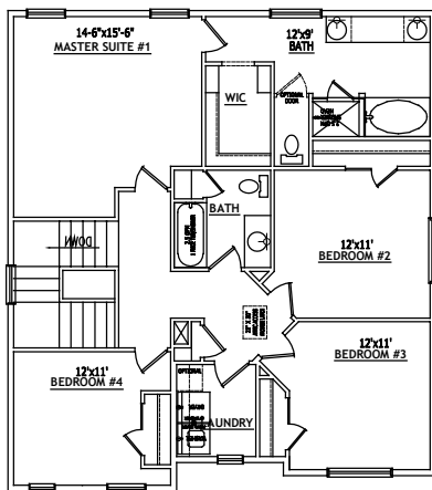
SECOND FLOOR PLAN 1,204 S.F.
