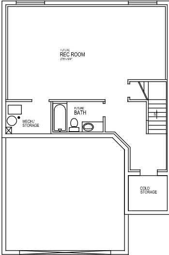
MAIN FLOOR PLAN 771 S.F.
