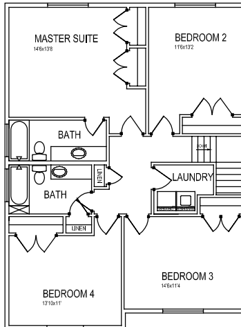
SECOND FLOOR PLAN 1157 S.F.
